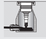
montaggio con cassaforma laterizio IP67 brick housing for recessed body IP67
