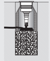
montaggio con cassaforma laterizio brick housing for recessed body
