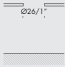
dimensione foro incasso opening dimensions for recessed
